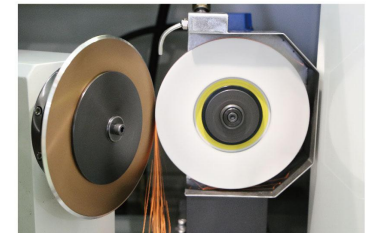
Grinding example of plane grinding wheel 平面砂輪研磨範例
