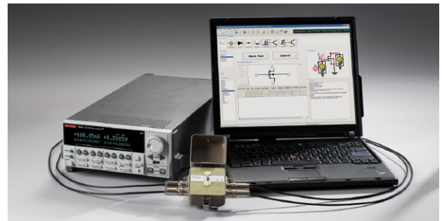
The flexible software architecture of ACS Basic Edition allows configuring systems with a wide range of controllers and test fixtures, as well as the exact number of SourceMeter SMU instruments the application requires.
